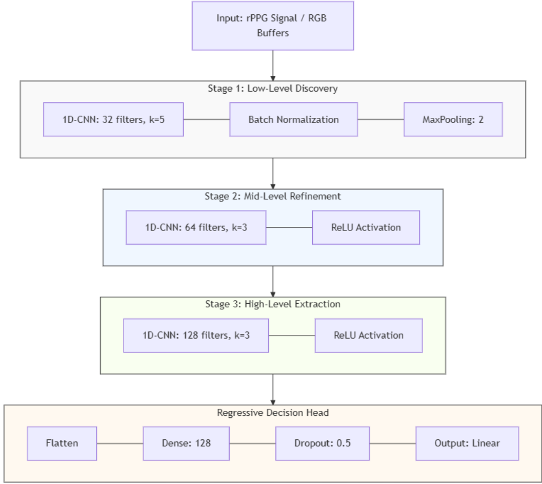
Figure 3 1D-CNN Architecture.
