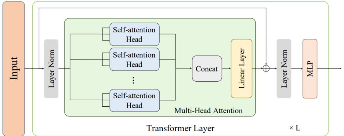
Figure 2 An illustration of a Transformer layer that is used in RADIANT
