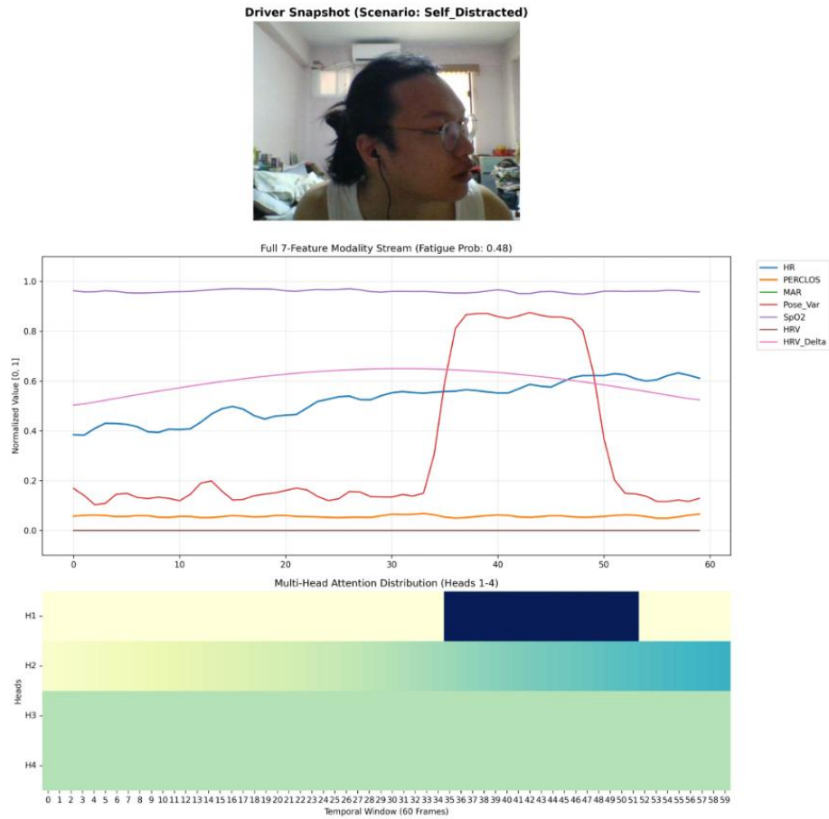
Figure 7 7-Feature Case Study.
